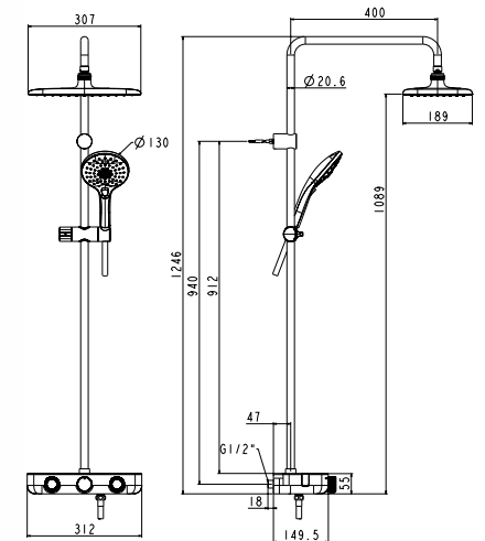
EasySET™ Exposed Auto Temperature Rainshower System
